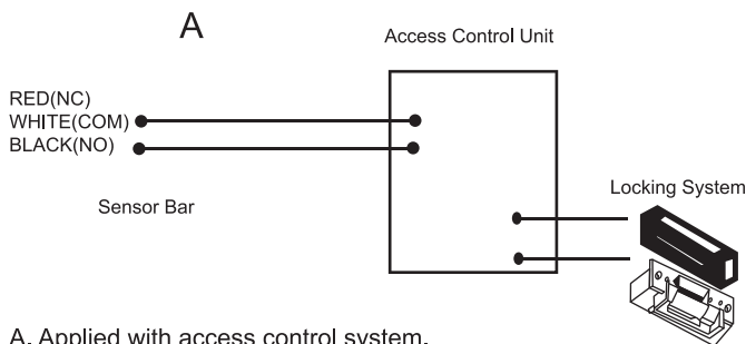
A. Applied with access control system. Press the sensor bar to activate the access control unit to open.
